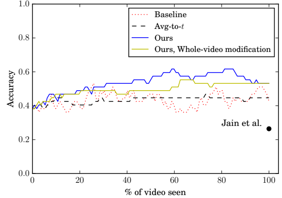
Figure 10: Classification performance on UCF Sports as a function of percentage of video seen. We present a baseline using only the current frame, as well as the average of frames from time 0 to t . Jain et al. [12] require the whole video. After only 20% of the video, the proposed model is already nearing its ultimate performance.
